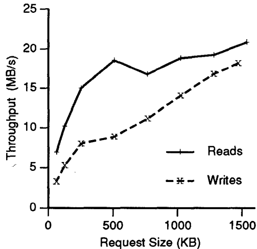
Figure 5: Hardware System Level Read and Write Performance. RAID-II achieves approximately 20 megabytes/second for both random reads and writes.
