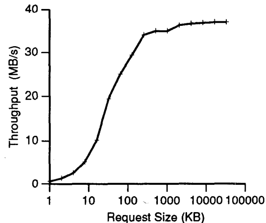
Figure 6: HIPPI Loopback Performance. RAID-II achieves 38.5 megabytes/second in each direction.
