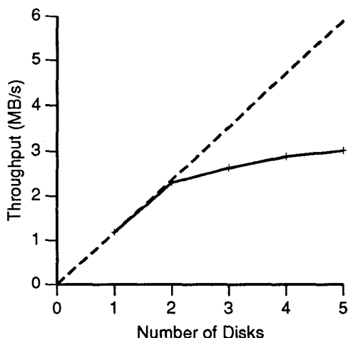
Figure 7: Disk read performance for varying number of disks on a single SCSI string. Cougar string bandwidth is limited to about 3 megabytes/second, less than that of three disks. The dashed line indicates the performance if bandwidth scaled linearly.
